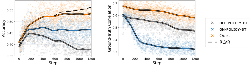
Figure 1: RL training on math data (DeepScaleR). We compare QWEN3-1.7B-BASE (Yang et al., 2025) optimized with three 4B RMs: \times ON-POLICY-BT , an on-policy trained BT RM; \times OFF-POLICY-BT , an off-policy BT RM given by SKYWORK-REWARD-V2-QWEN3-4B (Liu et al., 2026); and \times OURS , an RM trained with BONVOYAGE. All learned RMs are initialized from QWEN3-4B-BASE. Left: training accuracy as a function of RL step. The dashed curve corresponds to RLVR , and serves as a reference upper bound on the training accuracy attainable when the reward is perfectly faithful. Right: Pearson correlation between RM scores assigned to policy outputs at each RL step and their ground-truth correctness. We do not plot RLVR on the right because its reward is, by construction, perfectly correlated with correctness.
