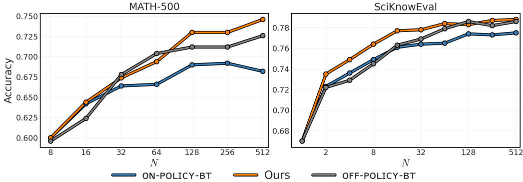
Figure 2: BoN scaling results. We evaluate RMs as rerankers for inference scaling by sampling N candidate responses from the base LM, scoring them with the RM, and selecting the highest-scoring response. All learned RMs are initialized from QWEN3-4B-BASE. Left: mathematics results on MATH-500, using QWEN3-1.7B-BASE as the base LM. We compare ON-POLICY-BT , an on-policy BT RM, OFF-POLICY-BT , the off-policy BT RM SKYWORK-REWARD-V2-QWEN3-4B, and Ours , an RM trained with BONVOYAGE. Right: science results on SCIKNOWEVAL, using QWEN3-1.7B-SCIENCE as the base LM. We compare ON-POLICY-BT and Ours .
